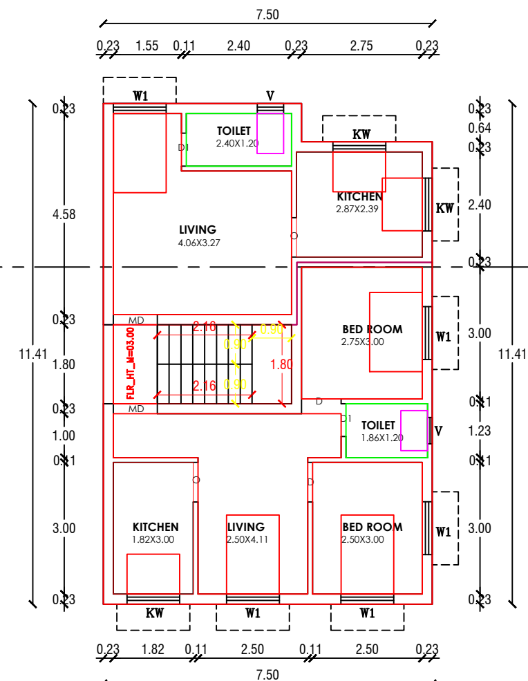
FIRST & SECOND FLOOR PLAN (PROPOSED)
