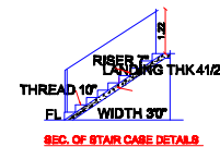
SEC. OF STAIR CASE DETAILS
