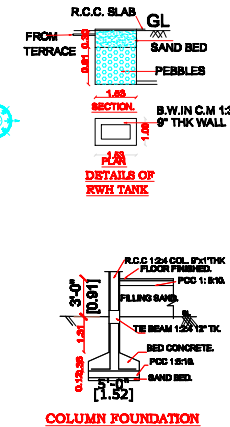
COLUMN FOUNDATION
