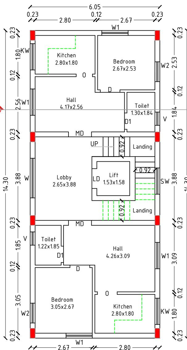
TYPICAL FLOOR PLAN FIRST & SECOND
