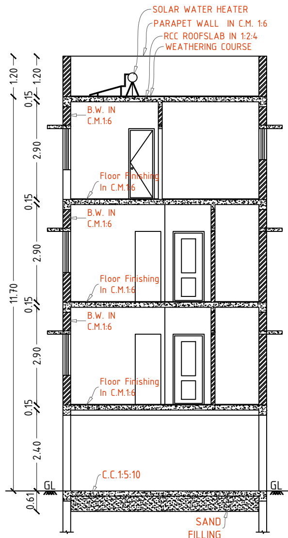
SECTION-A-A
