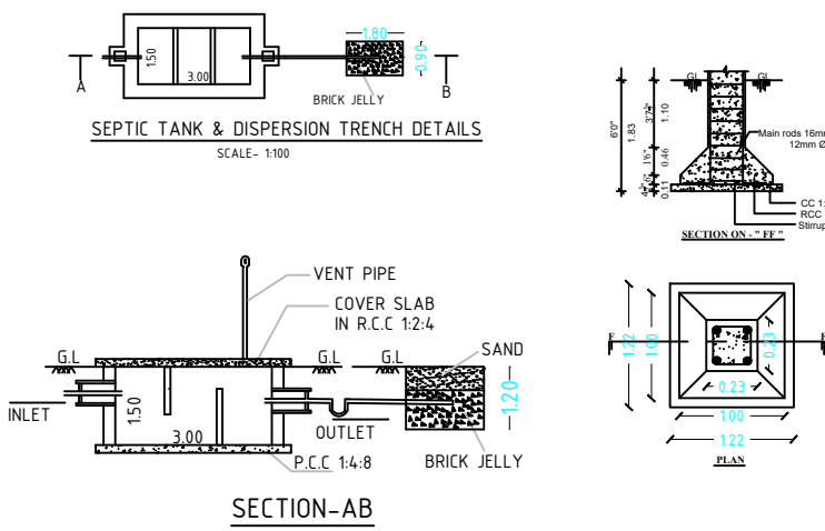
SECTION-AB
