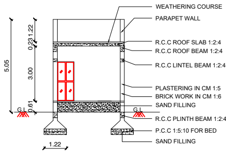
SECTION ON 'AA' (PROPOSED)
