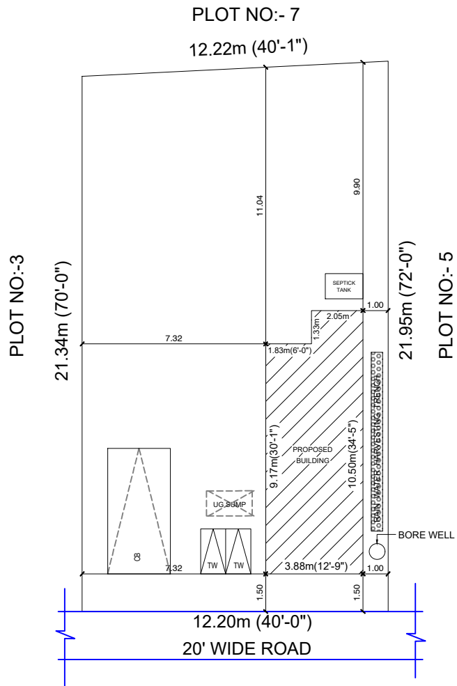
SITE PLAN (1:100) (PROPOSED)
