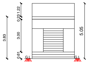
FRONT ELEVATION (PROPOSED)
