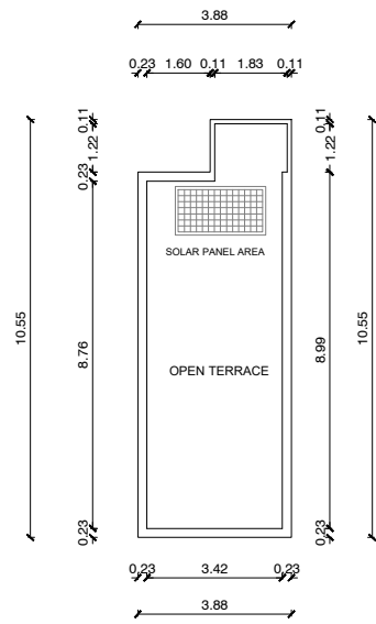
TERRACE FLOOR PLAN (PROPOSED)
