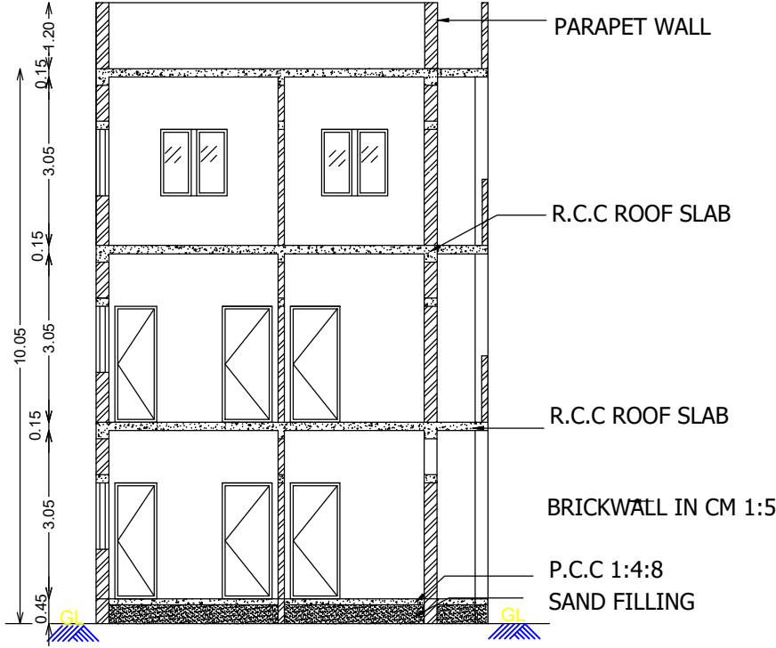
SECTION ELEVATION A-A
