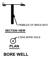
BORE WELL
