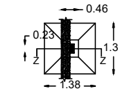
COLUMN FOOTING DETAIL
