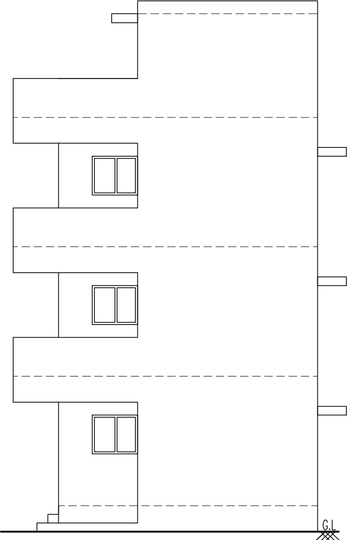
FRONT ELEVATION
