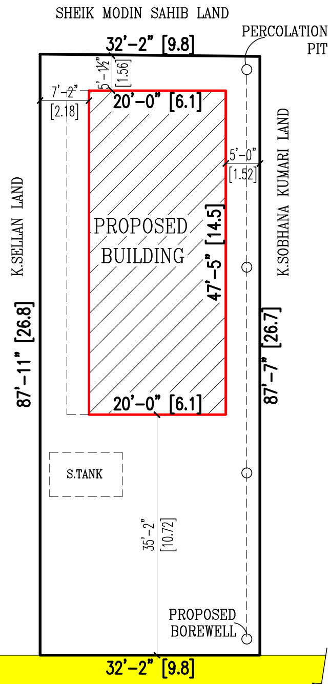
SITE PLAN
