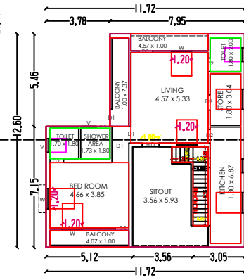
FIRST FLOOR SCALE 1:100
