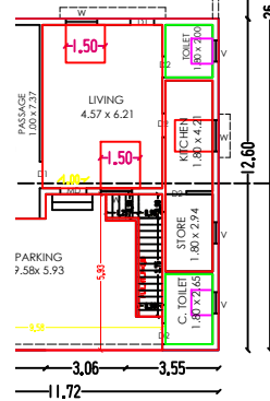
ROUND FLOOR SCALE 1:100
