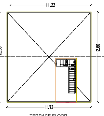
TERRACE FLOOR SCALE 1:100
