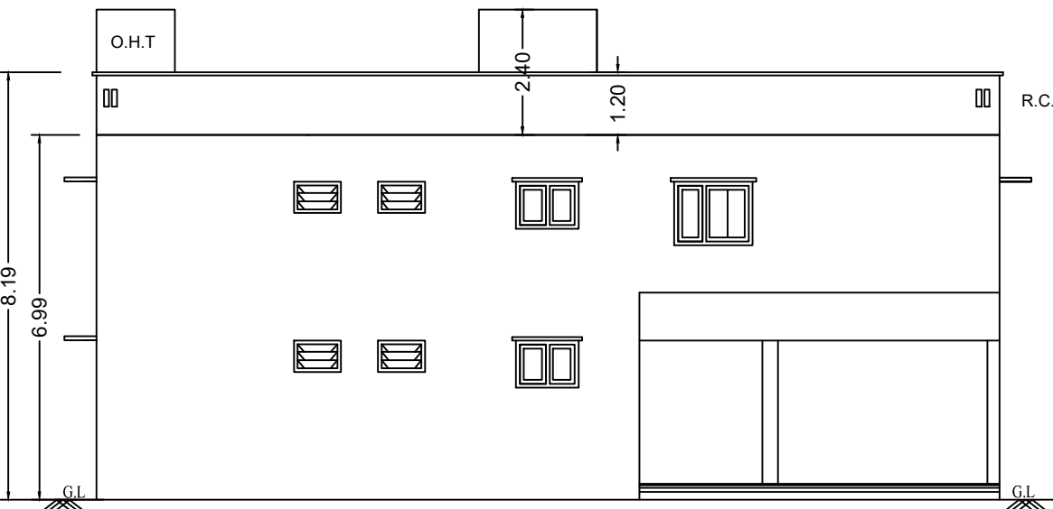
FRONT ELEVATION
