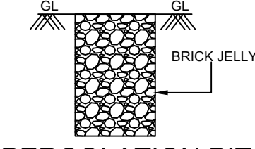
PERCOLATION PIT
