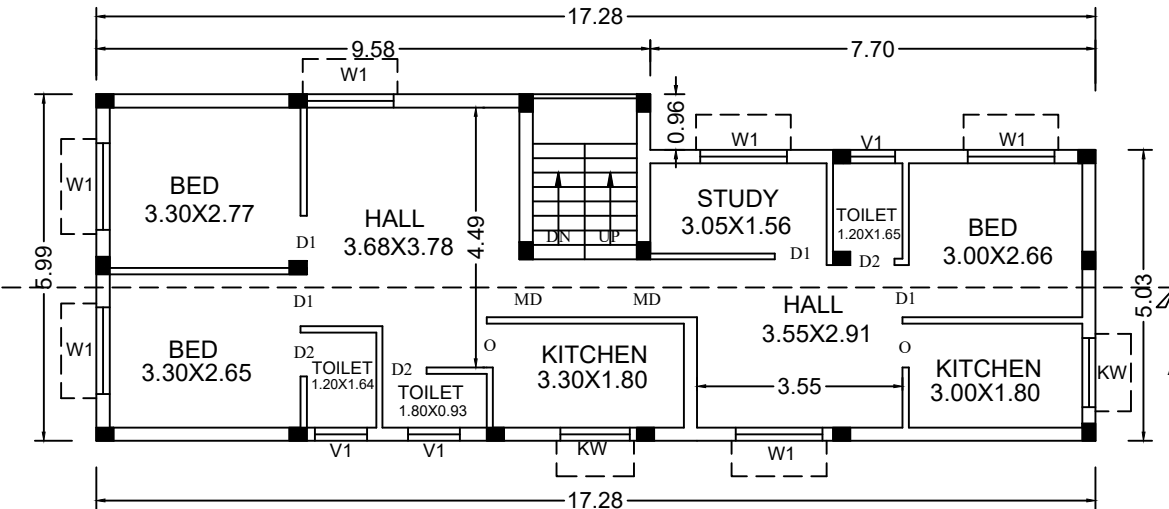
PRO.FIRST FLOOR PLAN
