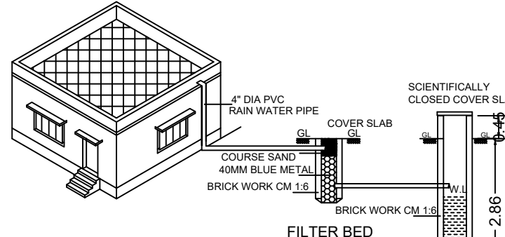
PROPOSED RAIN WATER SYSTEM WITH WELL DETAIL
