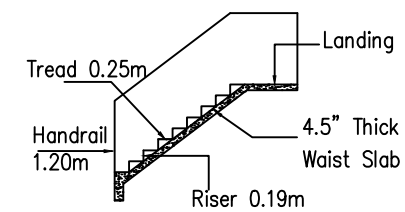
STAIRCASE DETAIL
