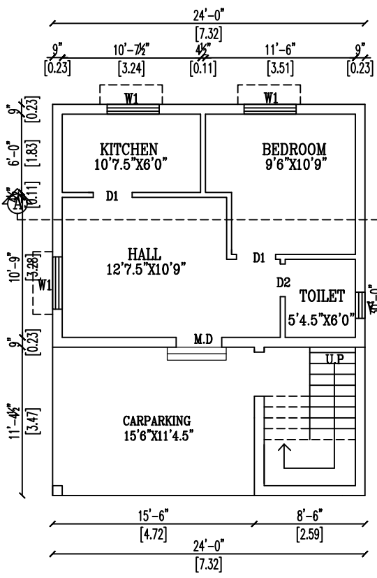
PRO. GROUND FLOOR PLAN
