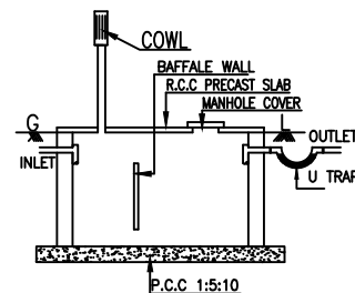
DETAILS OF SEPTIC TANK
