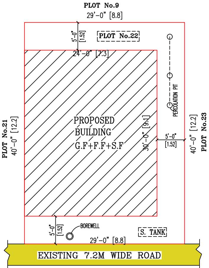
SITE PLAN
