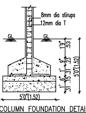
COLUMN FOUNDATION DETAIL
