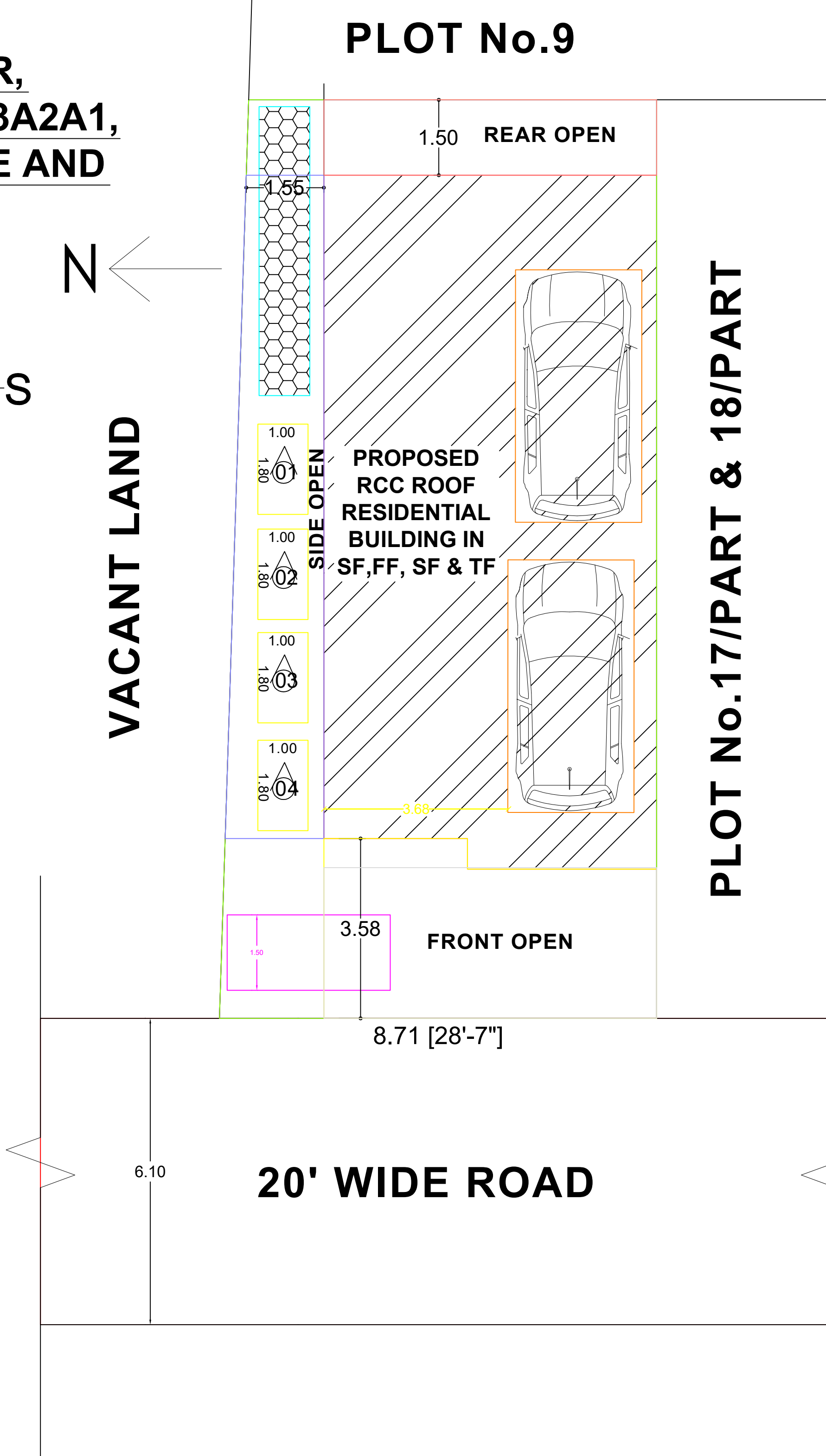
SITE PLAN [1:100]
