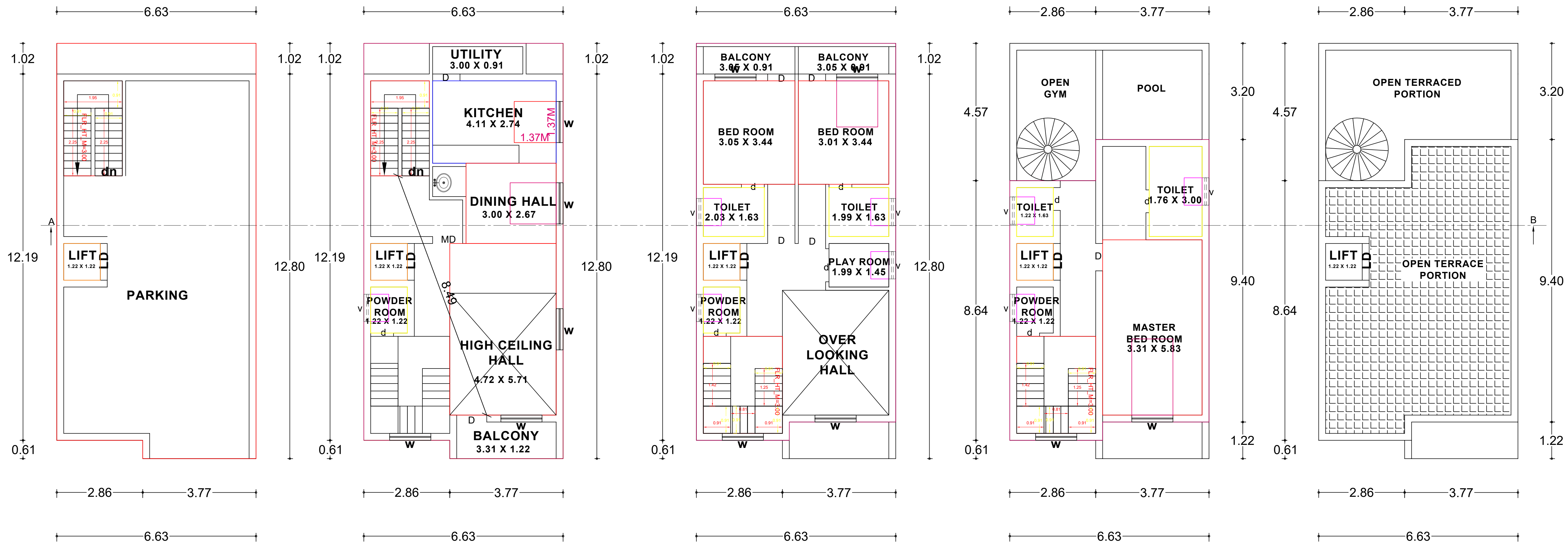
SLIT FLOOR PLAN
