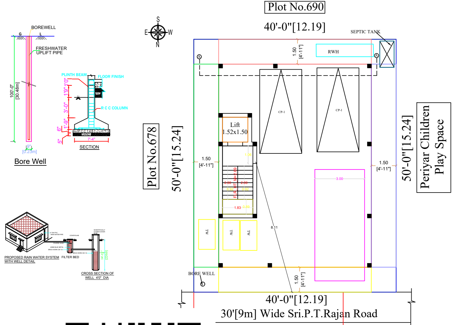
E CUM STILT FLOOR PLAN
