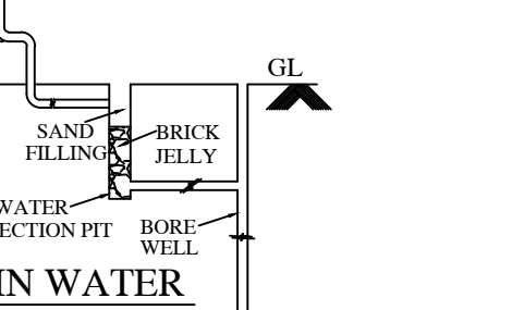
RAIN WATER COLLECTION PIT
