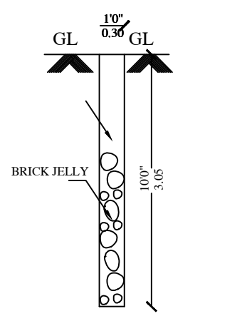
PERCOLATION PIT
