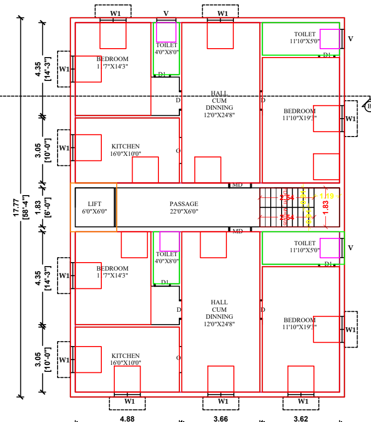
PROPOSED THIRD FLOOR PLAN
