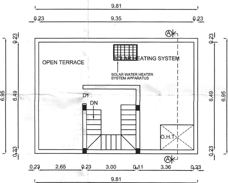
TERRACE FLOOR PLAN [PROPOSED]
