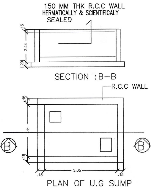
PLAN OF U.G. SUMP
