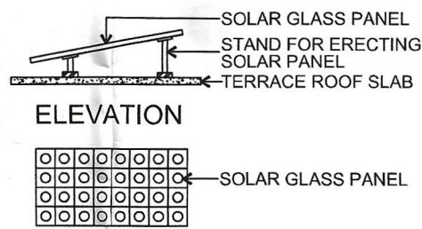
PLAN SOLAR PANEL DETAIL
