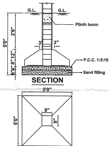
SECTION PLAN TYPICAL FOUNDATION DETAIL
