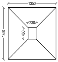
FOUNDATION DETAIL
