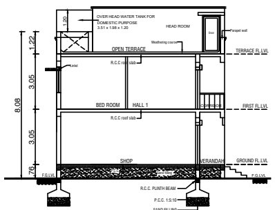
SECTION - AA' (PROPOSED)
