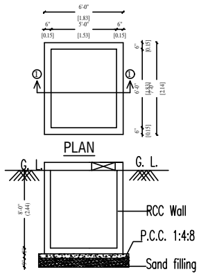
SECTION DETAIL OF SUMP (SCIENTIFICALLY SEALED)
