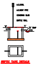
SEPTIC TANK DETAILS
