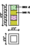
PERCOLATION TEST
