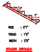
STAIRS DETAILS
