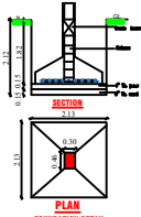
FOUNDATION DETAILS
