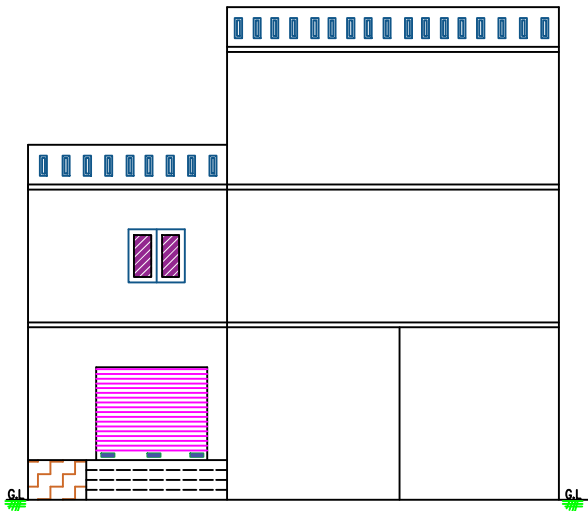
FRONT ELEVATION
