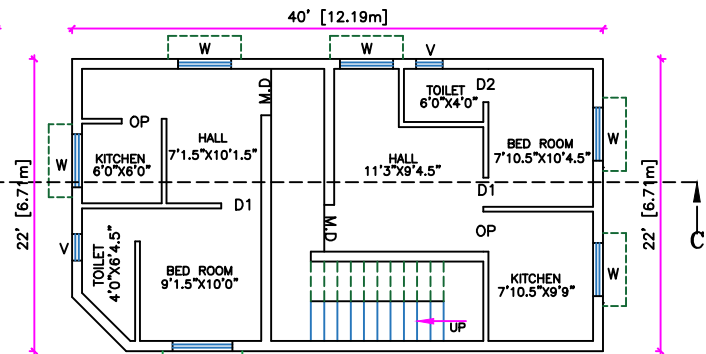
PRO.FIRST FLOOR PLAN
