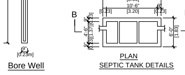
PLAN OF SEPTIC TANK DETAILS
