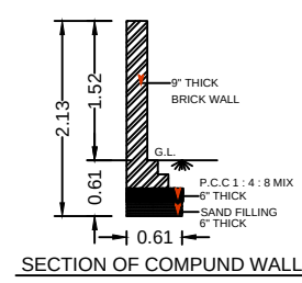
SECTION OF COMPOUND WALL
