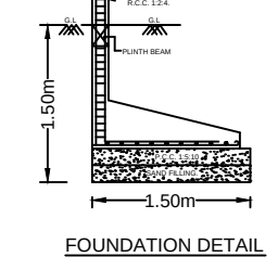
FOUNDATION DETAIL
