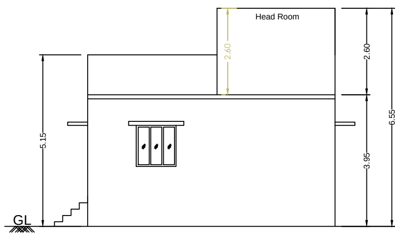
FRONT ELEVATION.
