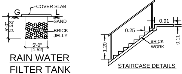
STAIRCASE DETAILS
