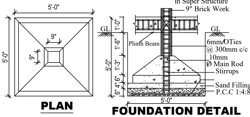
FOUNDATION DETAIL
