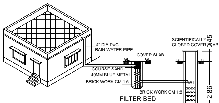
PROPOSED RAIN WATER SYSTEM WITH WELL DETAIL CROSS SECTION OF WELL 4'0" DIA
