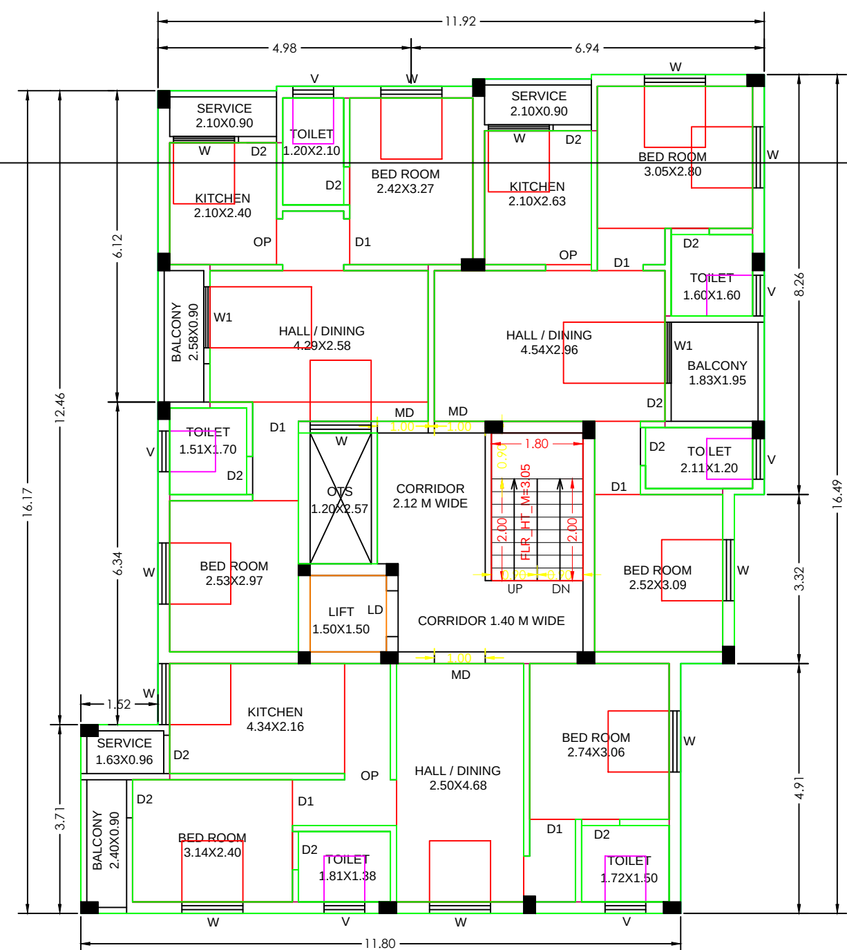
TYPICAL FLOOR PLAN=1,2 TYPICAL FLOOR PLAN=1,2
