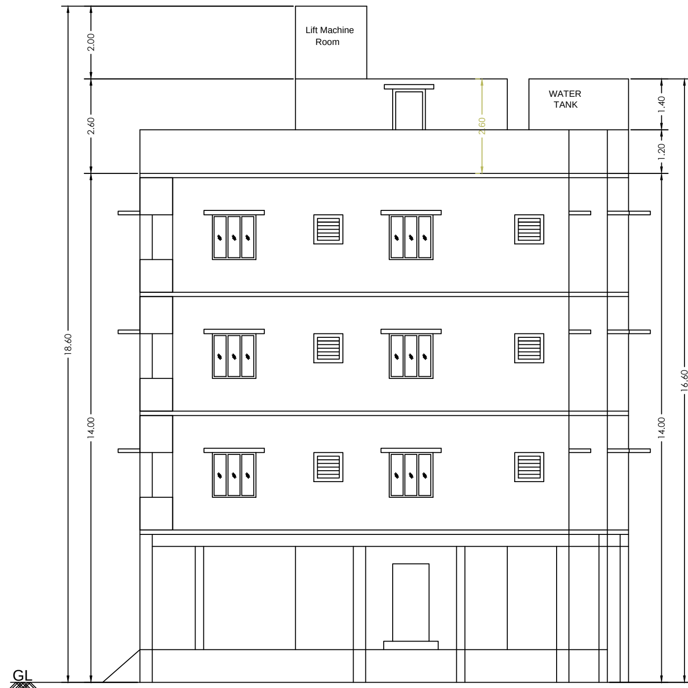
FRONT ELEVATION (NORTHERN SIDE).
