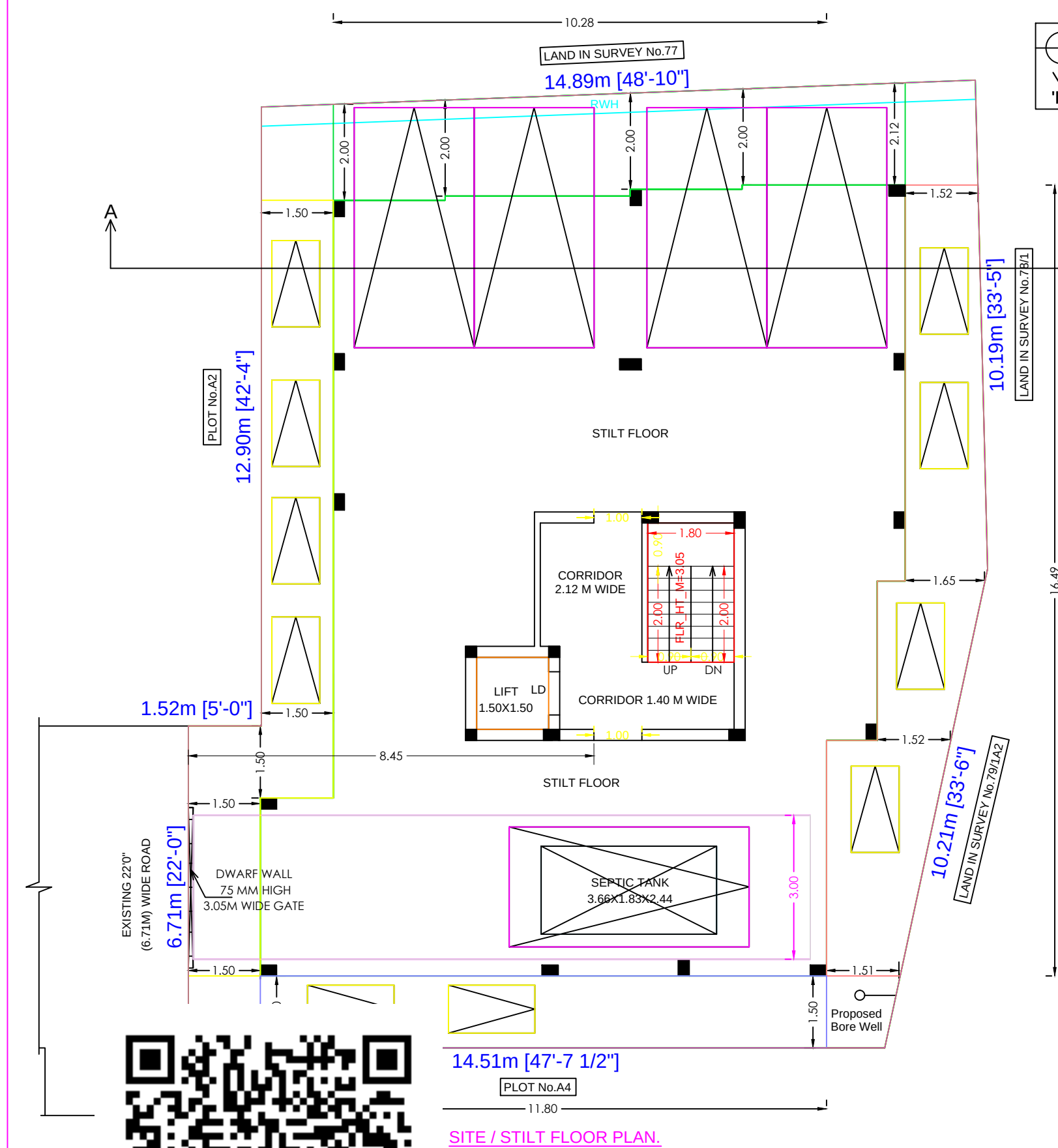
SITE / STILT FLOOR PLAN.
