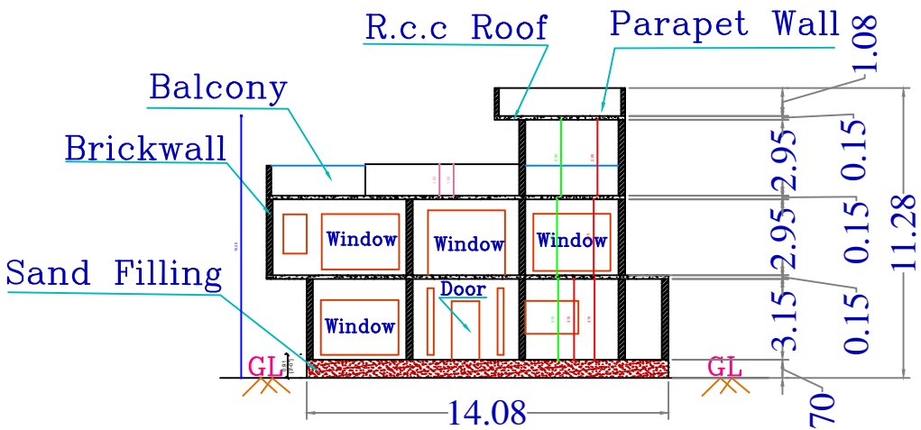
EASTEN SIDE SECTION A'A'
