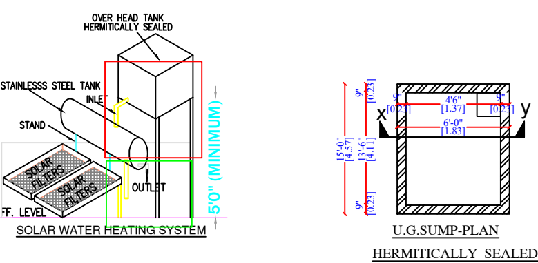
U.G. SUMP-PLAN HERMITICALLY SEALED
