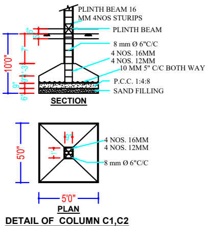
DETAIL OF COLUMN C1,C2
