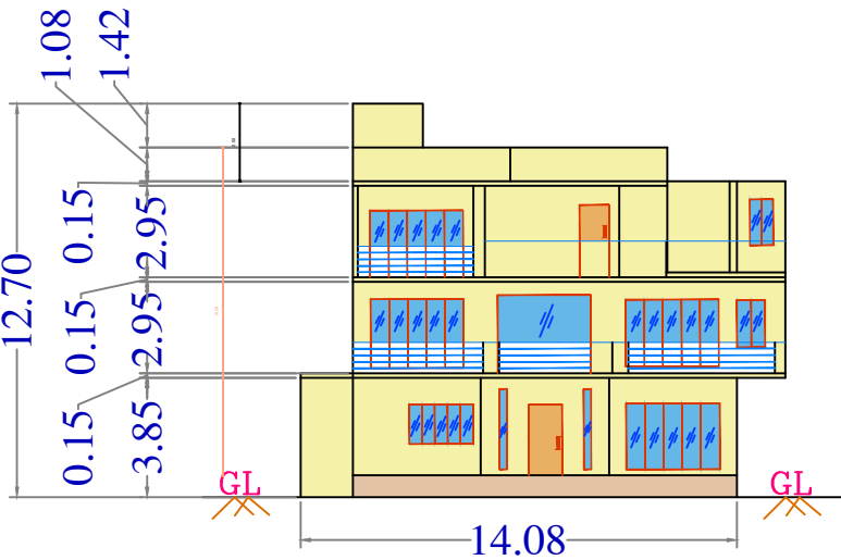
EASTEN SIDE ELEVATION
