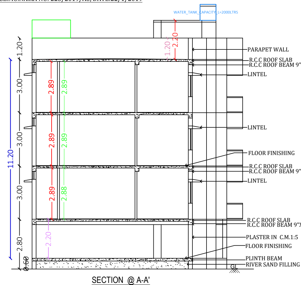
SECTION @ A-A'
