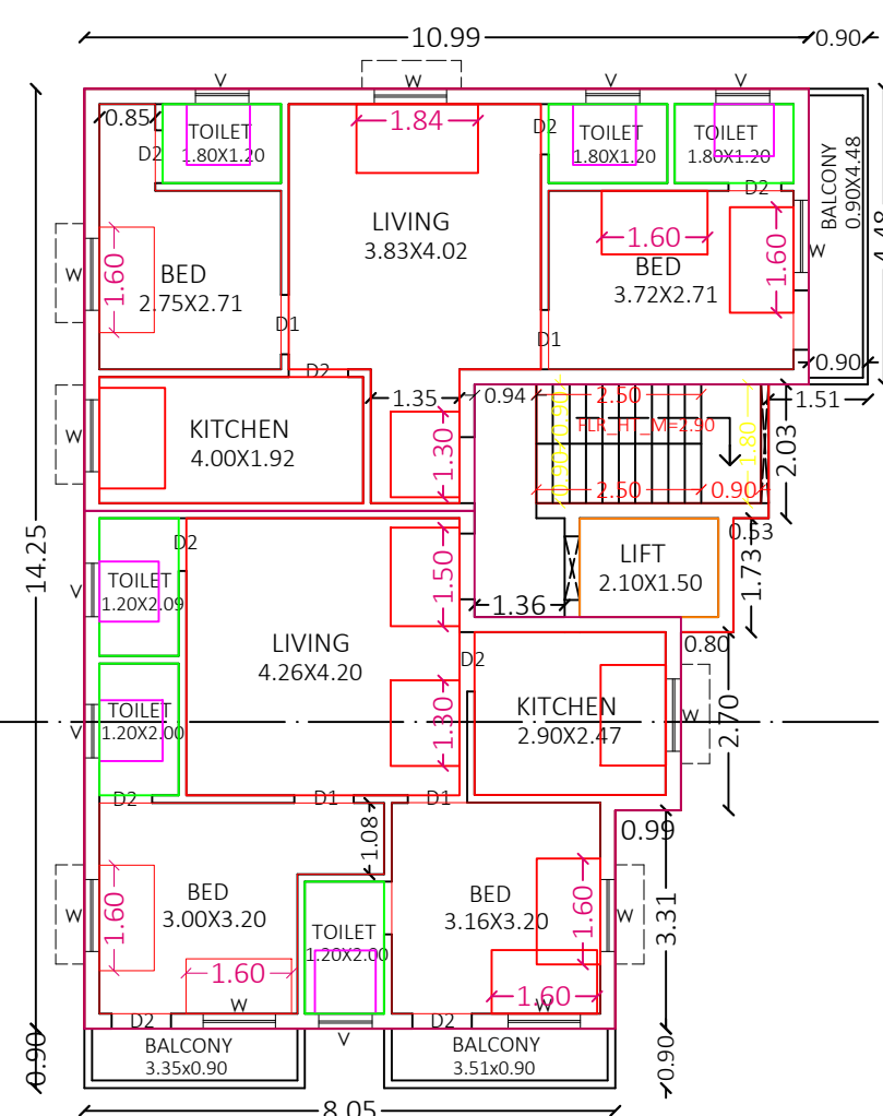
SECOND FLOOR
