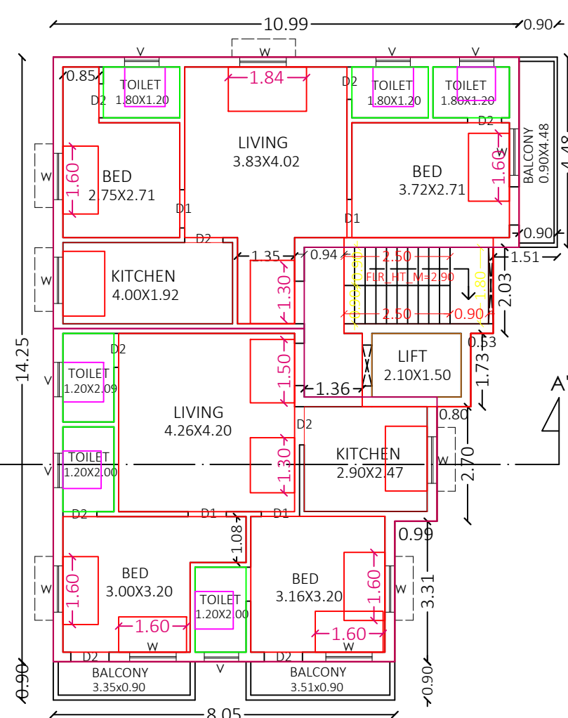
THIRD FLOOR
