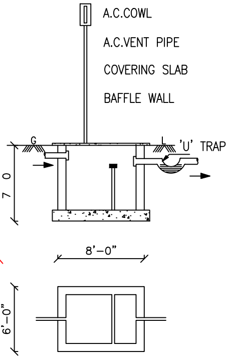
SEPTIC TANK
