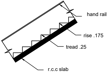
STAIR
