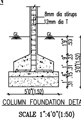
SCALE 1"=4'0"(1:50)
