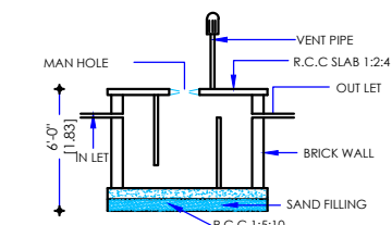
SECTION 2.1 SEPTIC TANK DETAIL
