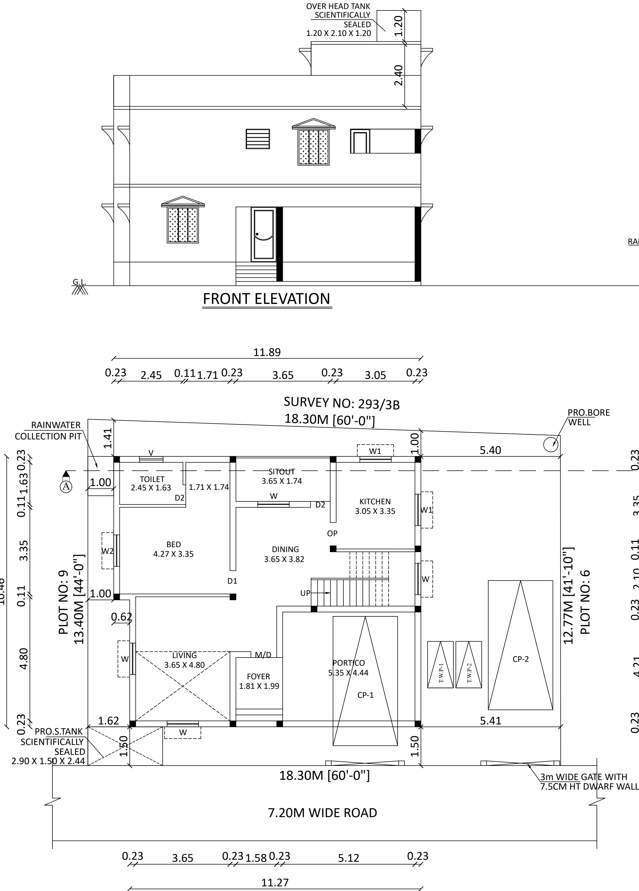
SITE CUM PRO.GROUND FLOOR PLAN
