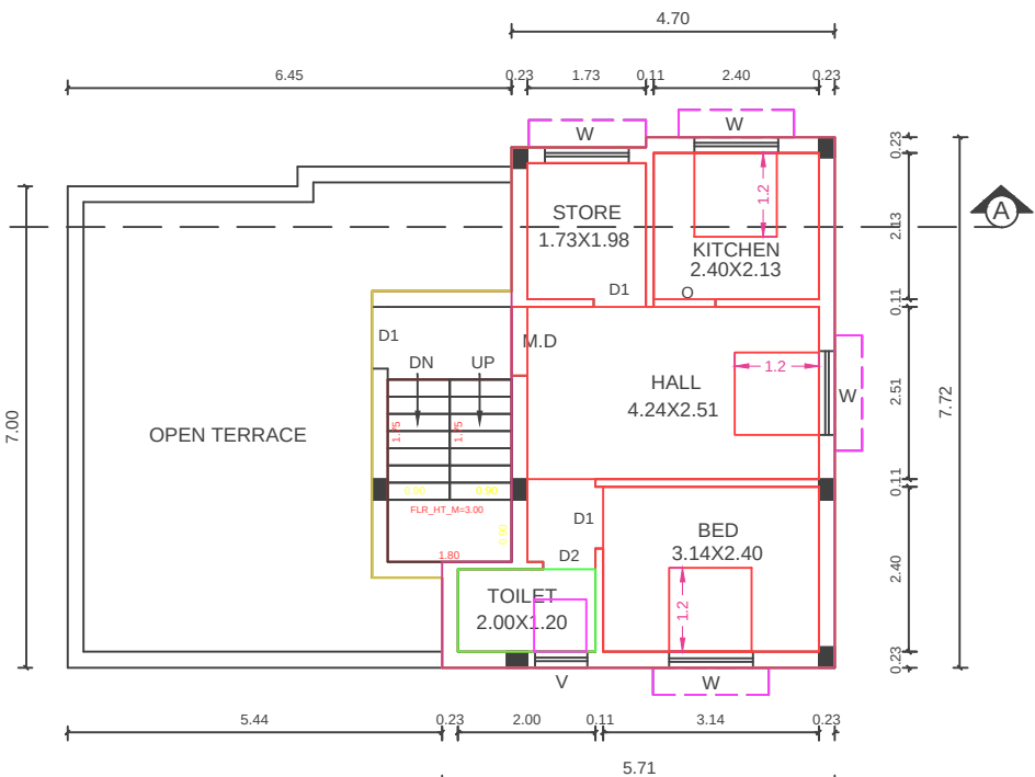
SECOND FLOOR PLAN (PART)
