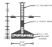
FOUNDATION DETAILS
