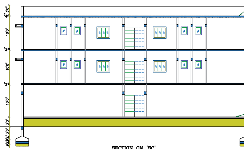
SECTION ON 'SC'
