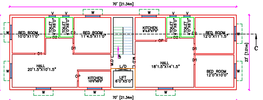
PRO.SECOND FLOOR PLAN
