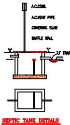
SEPTIC TANK DETAILS
