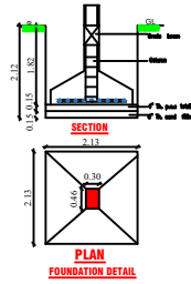
FOUNDATION DETAIL
