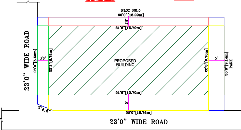
SITE PLAN SCALE 1"=8'0"
