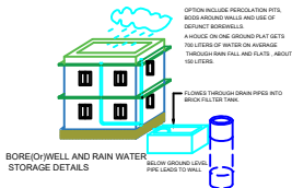
BOREHOLE/WELL AND RAIN WATER STORAGE DETAILS
