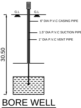
BORE WELL
