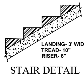
STAIR DETAIL
