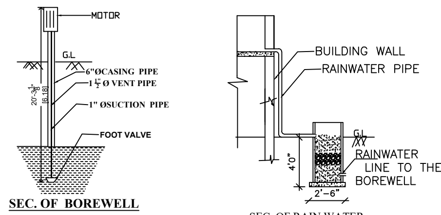
SEC. OF RAIN WATER HARVEST
