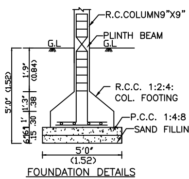
FOUNDATION DETAILS
