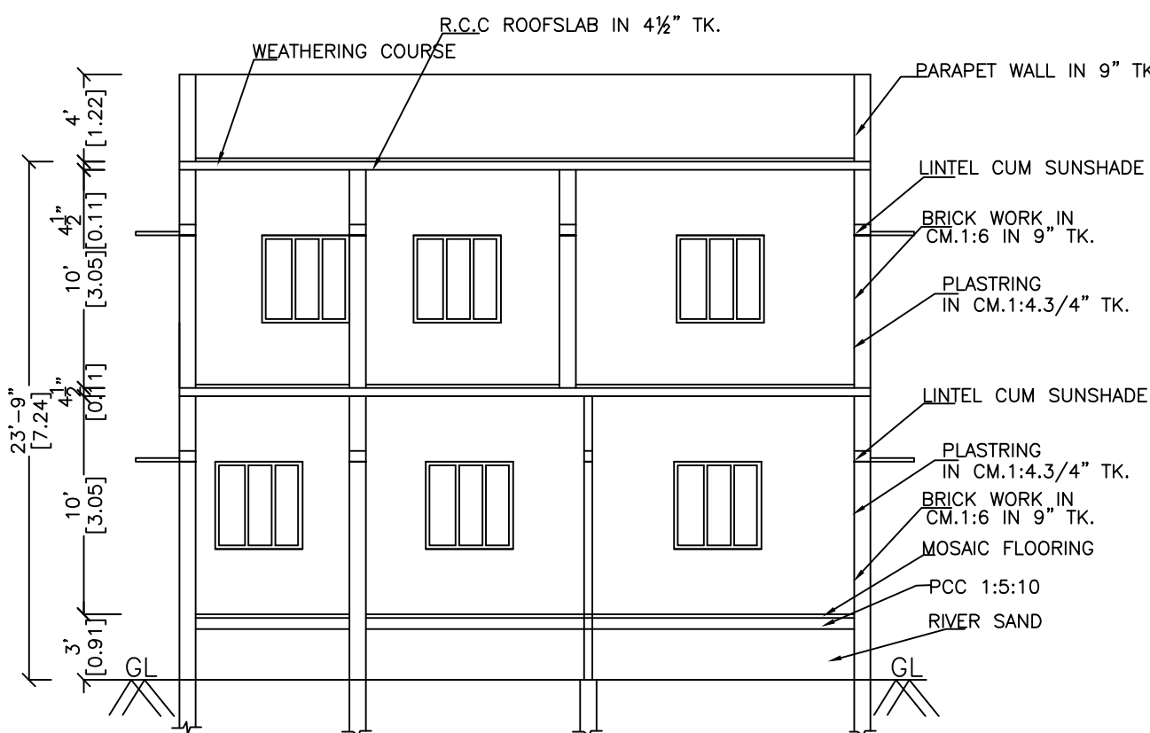
SECTION-"AB"
