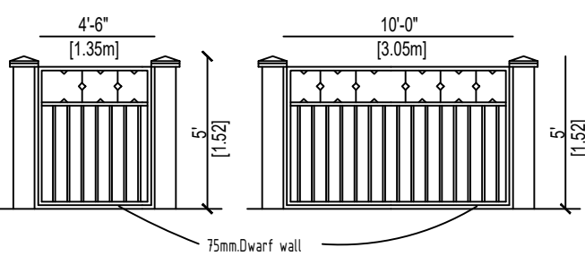
GATE ELEVATION (NTS)
