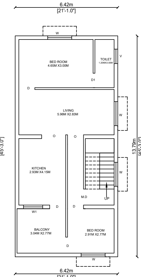
EXISTING APPROVED FIRST FLOOR PLAN
