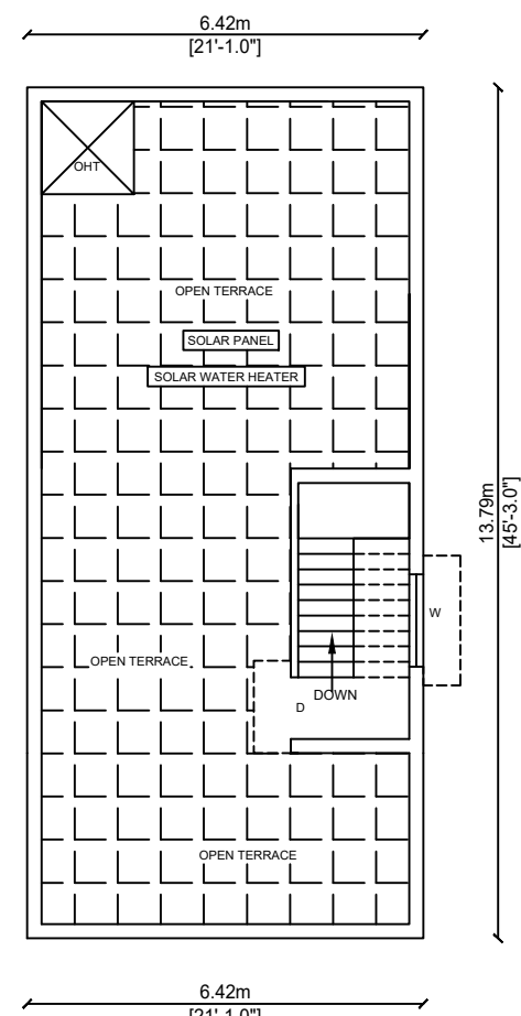
PROPOSED TERRACE FLOOR PLAN
