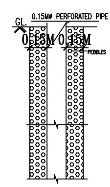
PLAN BORE WELL "nts"
