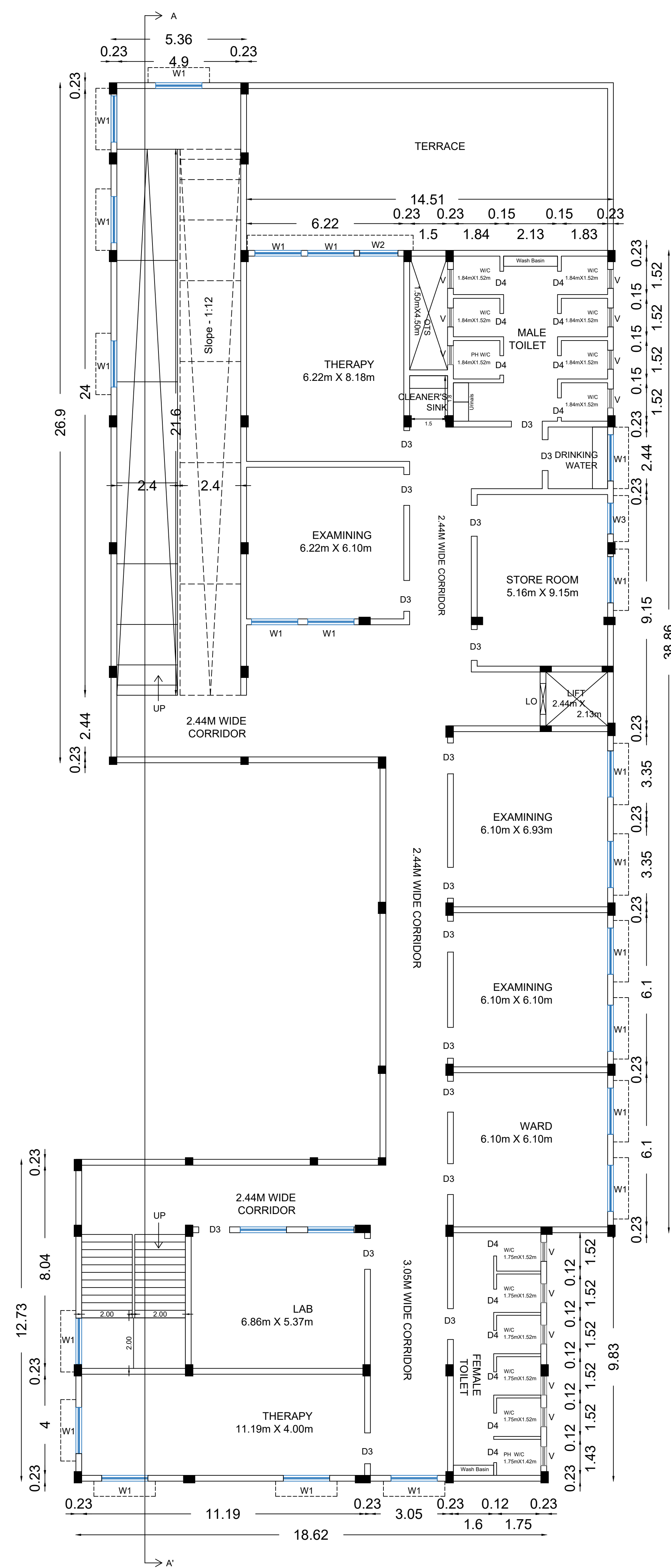
FIRST FLOOR
