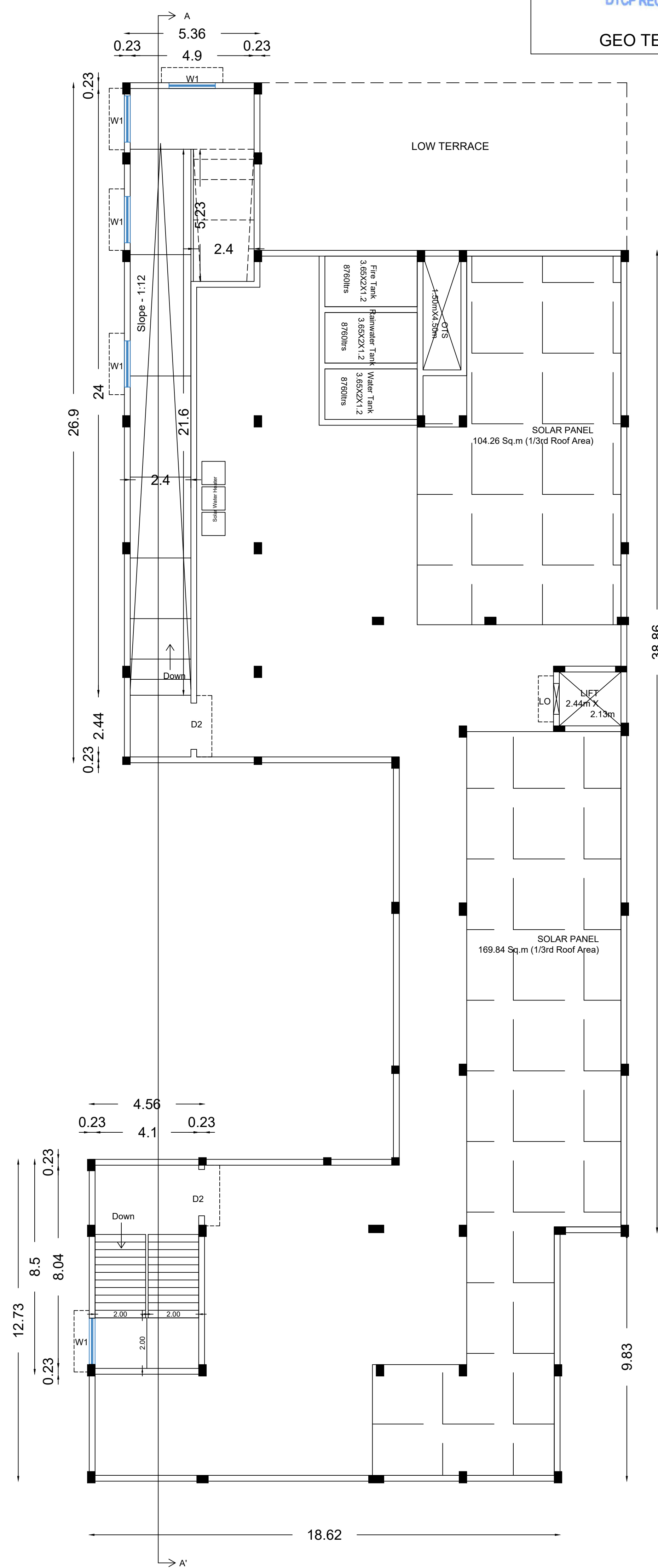
TERRACE FLOOR
