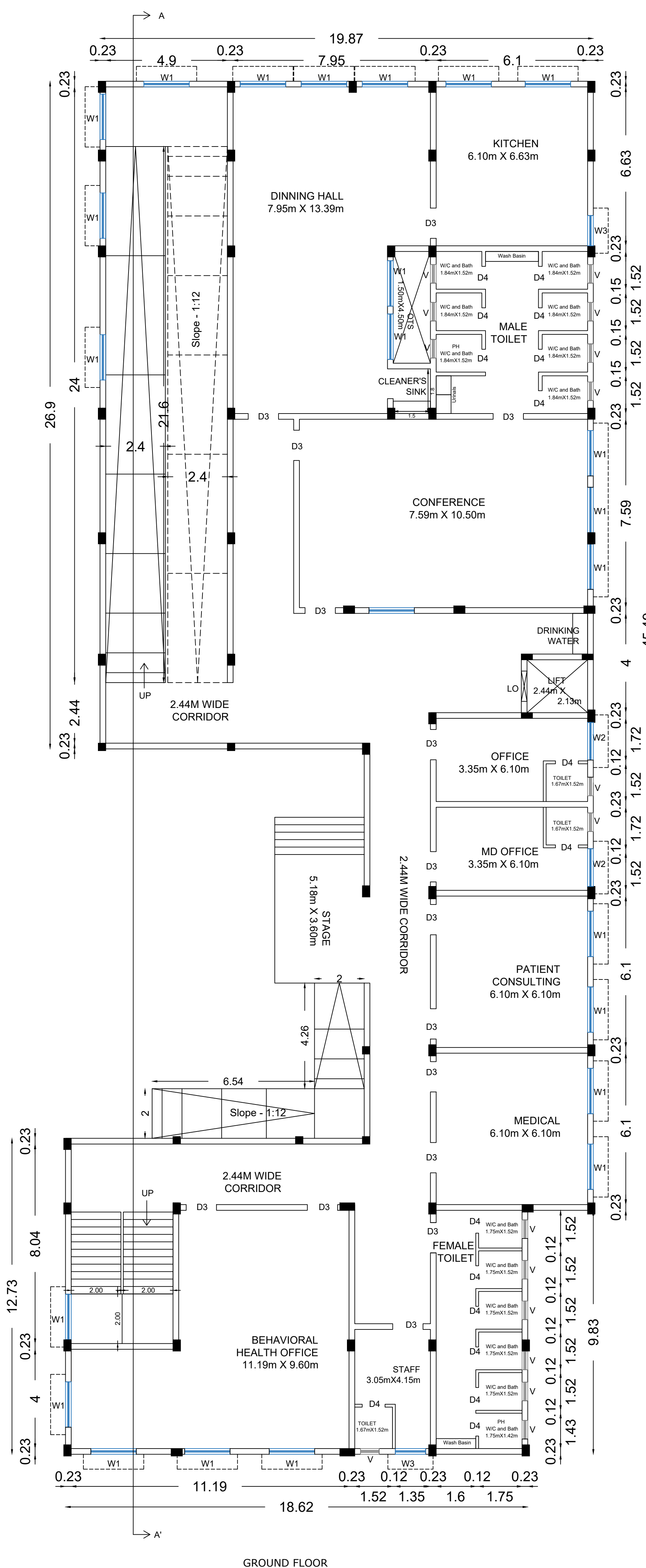
GROUND FLOOR
