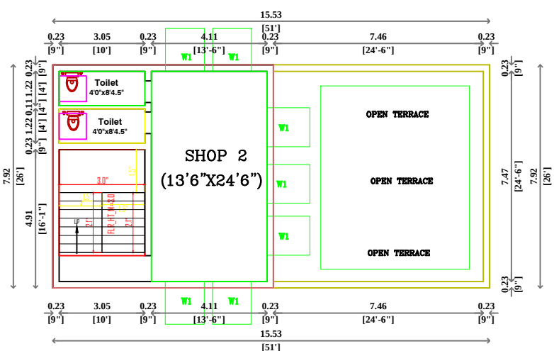
PROPOSED FIRST FLOOR PLAN (COMMERCIAL)
