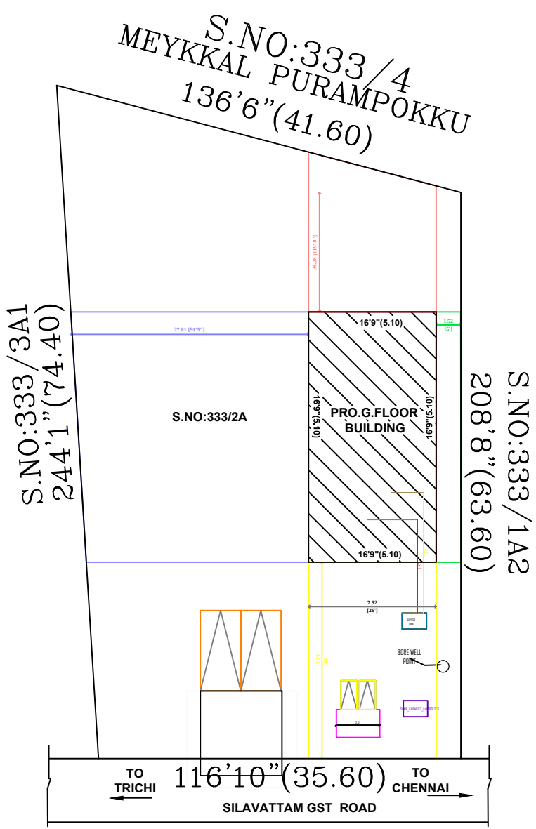
SITE&KEY PLAN
