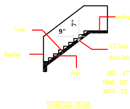
STAIRCASE DETAIL
