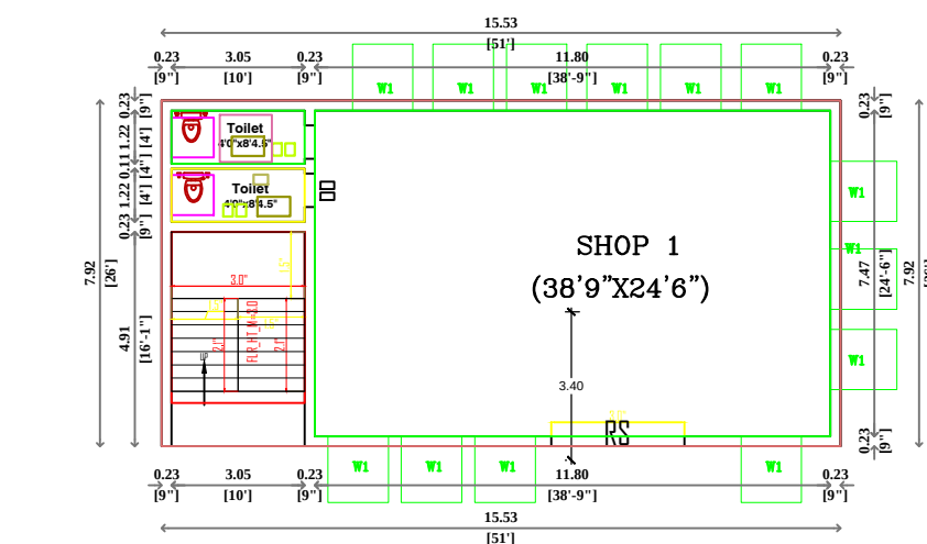
PROPOSED GROUND FLOOR PLAN (COMMERCIAL)
