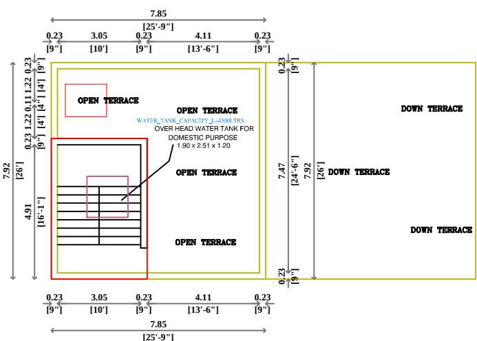
PROPOSED TERRACE FLOOR PLAN (COMMERCIAL)
