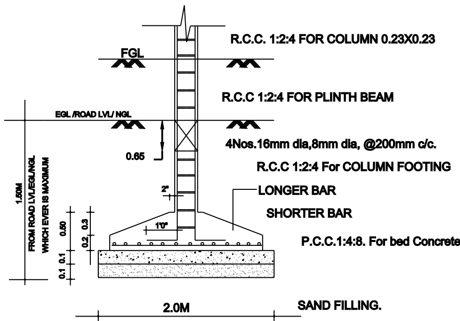
FOUNDATION DETAILS
