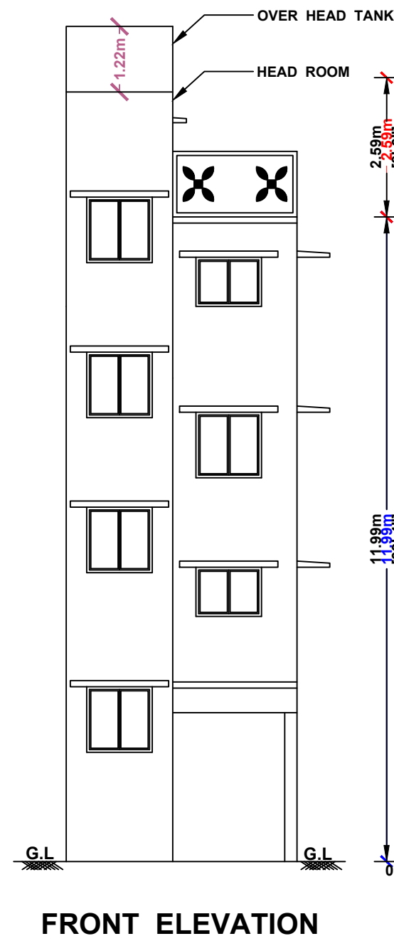
FRONT ELEVATION
