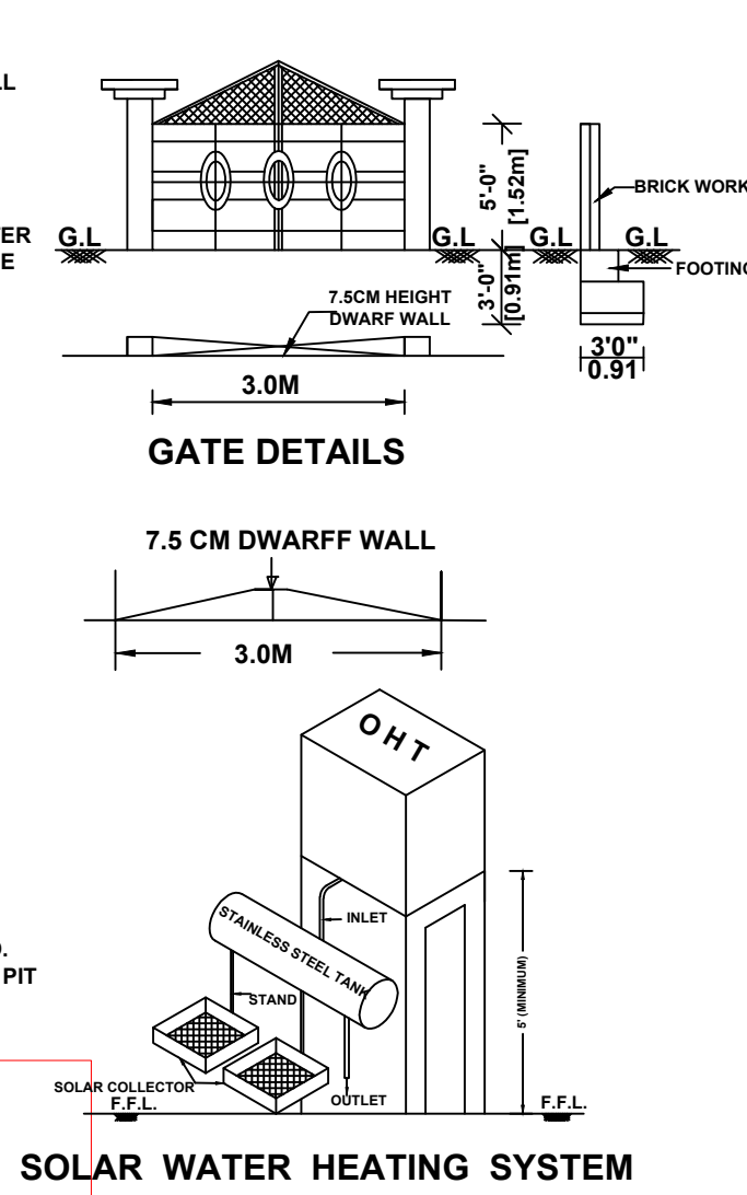
SOLAR WATER HEATING SYSTEM
