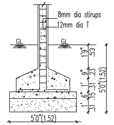
COLUMN FOUNDATION DETAIL SCALE 1"=4'0"(1:50)
