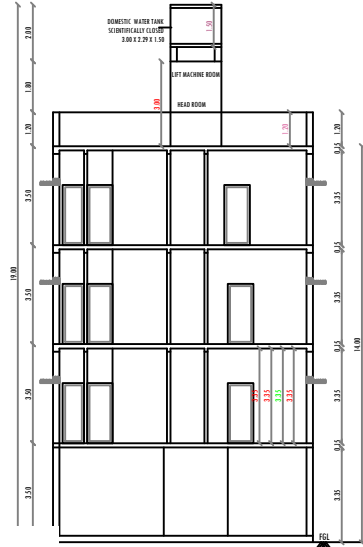
SECTION ON 'A-A' (PROPOSED)
