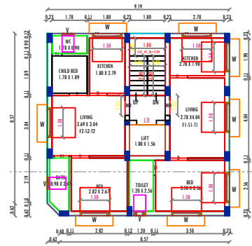
TYPICAL-FIRST, SECOND & THIRD FLOOR PLAN (PROPOSED)
