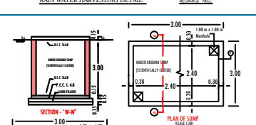
SECTION 'W-W' (PROPOSED)
