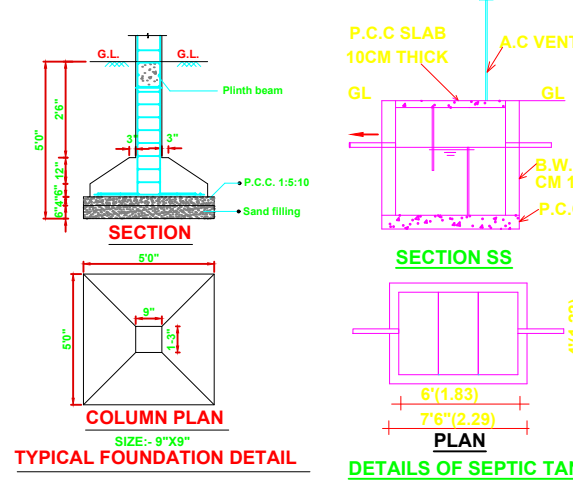
TYPICAL FOUNDATION DETAIL
