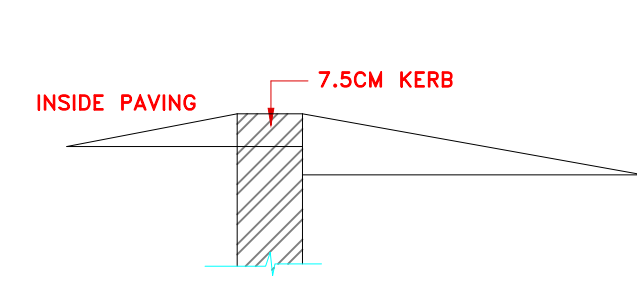
DWARF WALL SECTION
