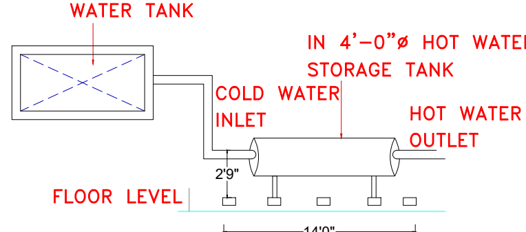
Solar Waterheater Detail
