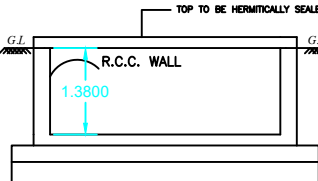
RWH SECTION (SAMPLE) RWH_CAPACITY_L=5000LTRS
