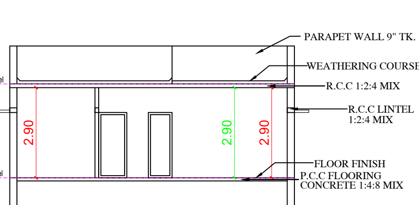
SECTION - AA (PROPOSED)
