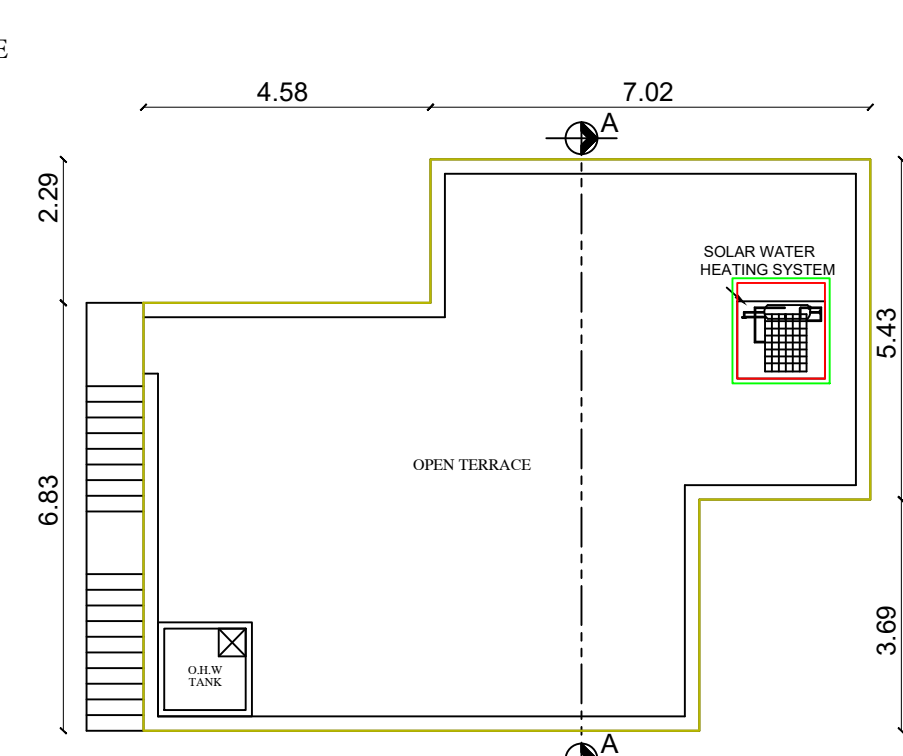
TEERACE FLOOR PLAN (PROPOSED)
