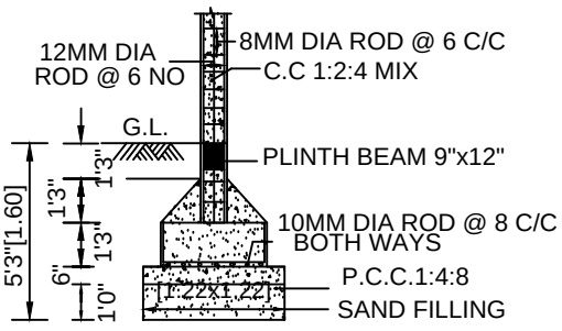
RUN THROUGH COLUMN FOUNDATION SCALE 1"=4'0" (1:50)
