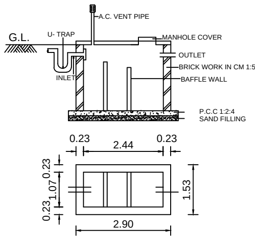
SEPTIC TANK DETAIL
