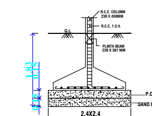
FOUNDATION DETAIL
