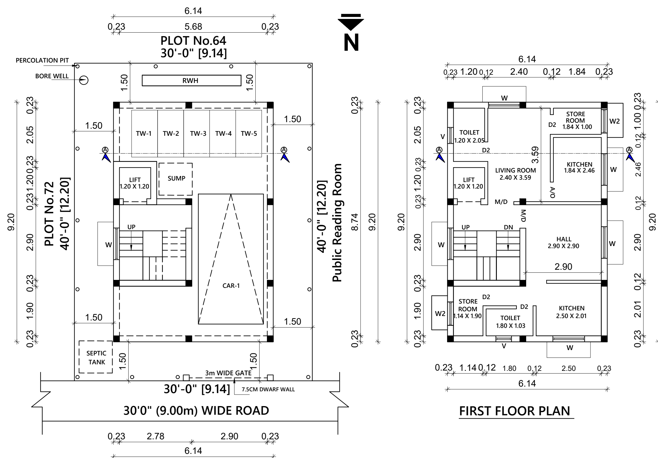
SITE cum STILT FLOOR PLAN
