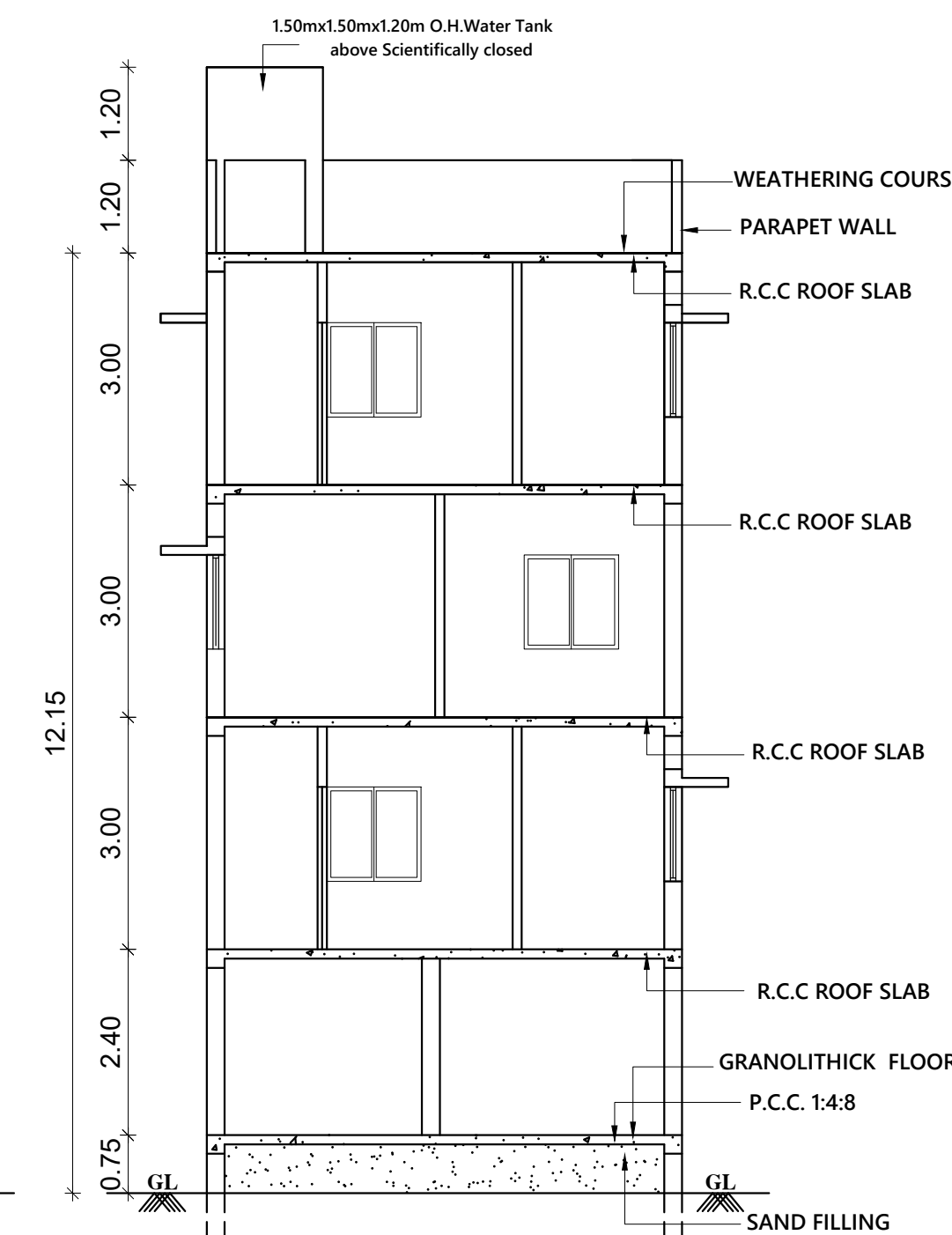
SECTION- AA
