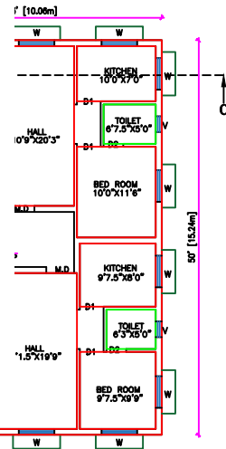
TYPICAL FIRST & SECOND FLOOR PLAN
