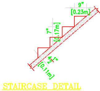
STAIRCASE DETAIL
