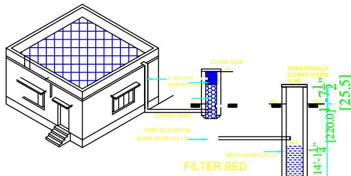
PROPOSED RAIN WATER SYSTEM WITH WELL DETAIL
