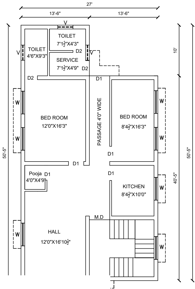
R PLAN
