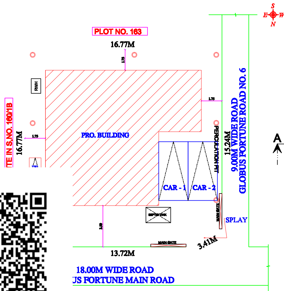
SITE PLAN
