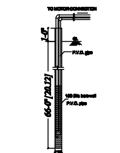
SECTION OF SEPTIC TANK
