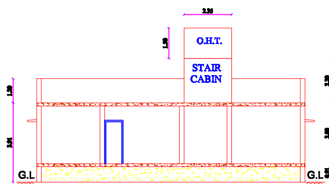
SECTION ON A-A (PROPOSED)
