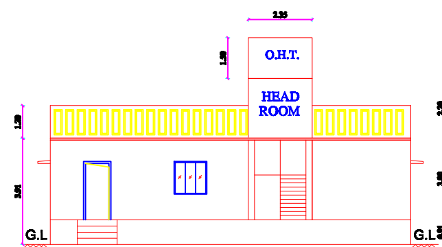
FRONT ELEVATION (PROPOSED)
