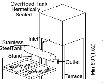
SEC. OF RAIN WATER HARVEST
