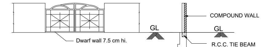
COMPOUND WALL DETAILS
