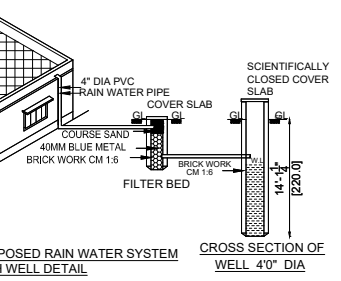
PROPOSED RAIN WATER SYSTEM WITH WELL DETAIL
