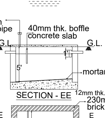
SECTION - EE
