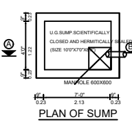
PLAN OF SUMP
