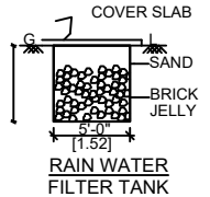
RAIN WATER FILTER TANK
