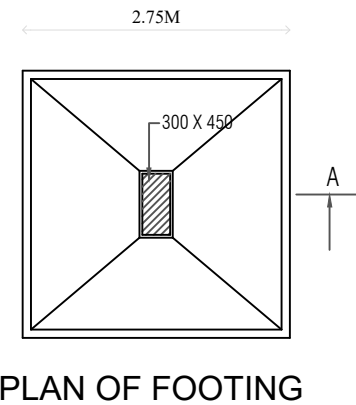
PLAN OF FOOTING
