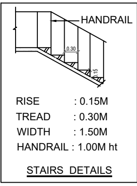
STAIRS DETAILS
