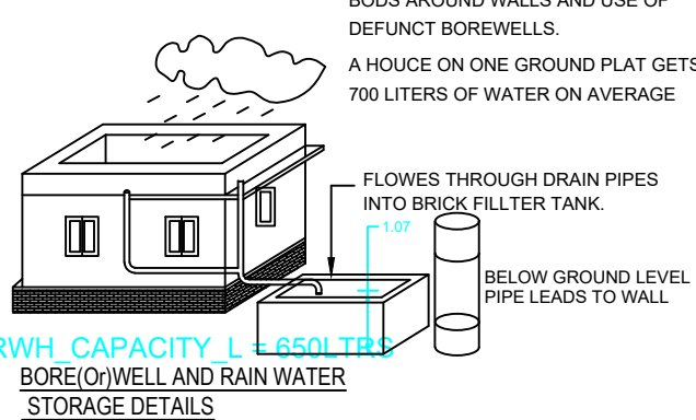
BOREWELL AND RAIN WATER STORAGE DETAILS
