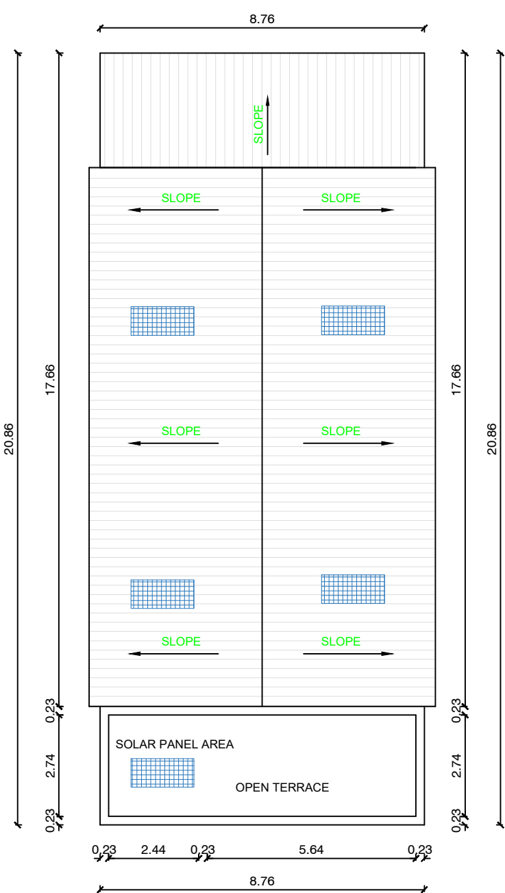
TERRACE FLOOR PLAN (PROPOSED)
