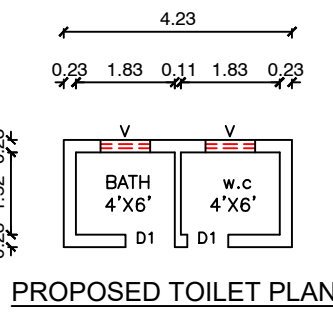
PROPOSED TOILET PLAN
