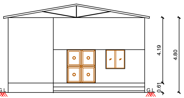
FRONT ELEVATION (PROPOSED)
